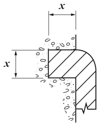
membranes less than 10mm thick formed in-situ
