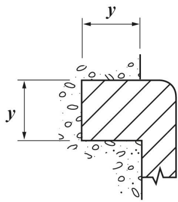
membranes greater than 10mm thick formed in-situ
