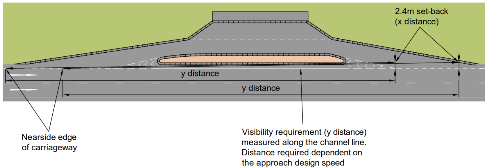
Figure 3.16 Visibility requirements at the exit from type A parking lay-bys with a merge taper
