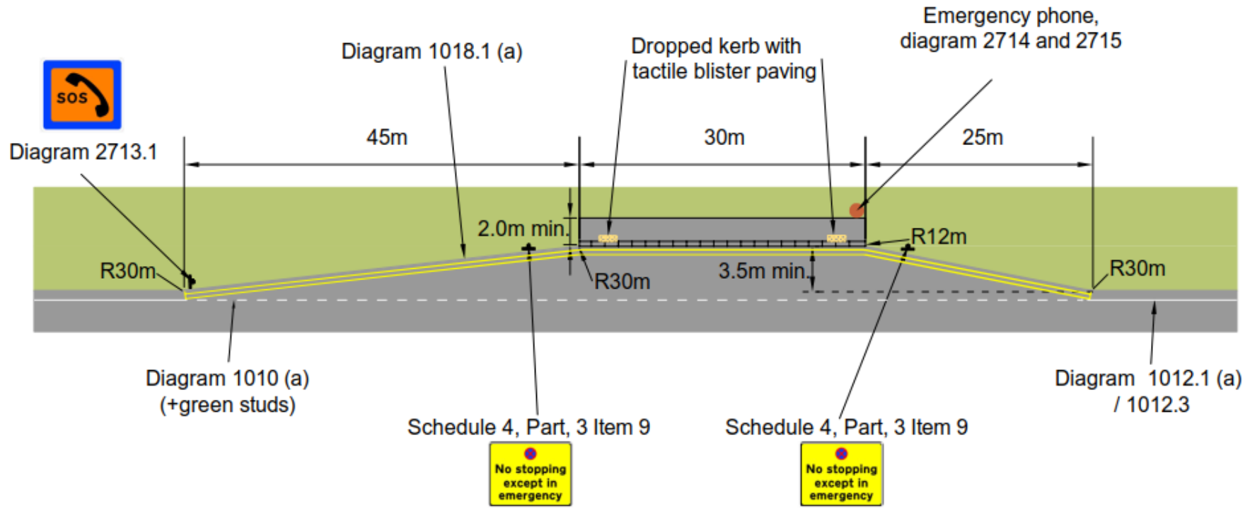
Figure 6.2N3 Geometric layout of emergency lay-by
