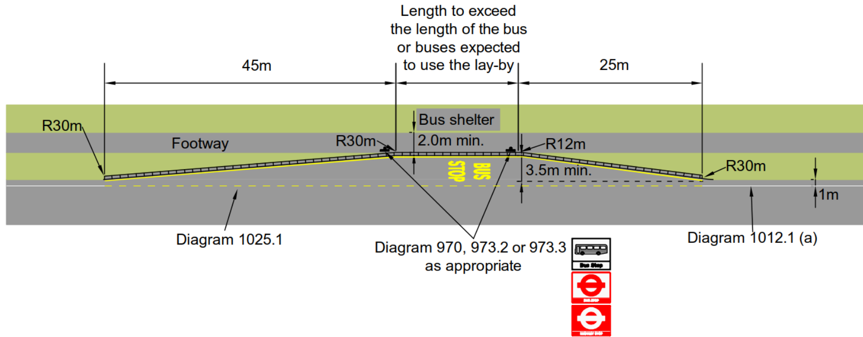
Figure 5.6N Geometric layout of a bus lay-by
