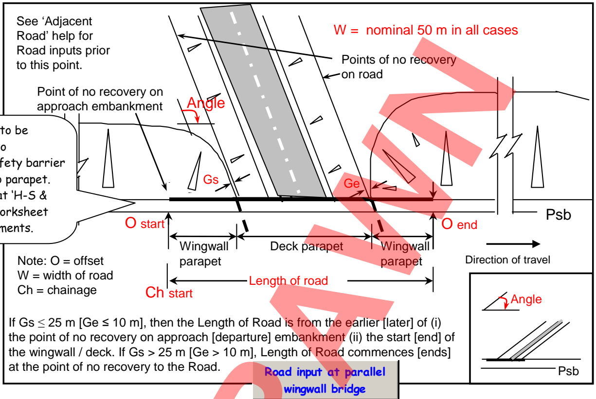
Figure 5.15 (e) Road crossing under Road at structure with parallel wingwalls
