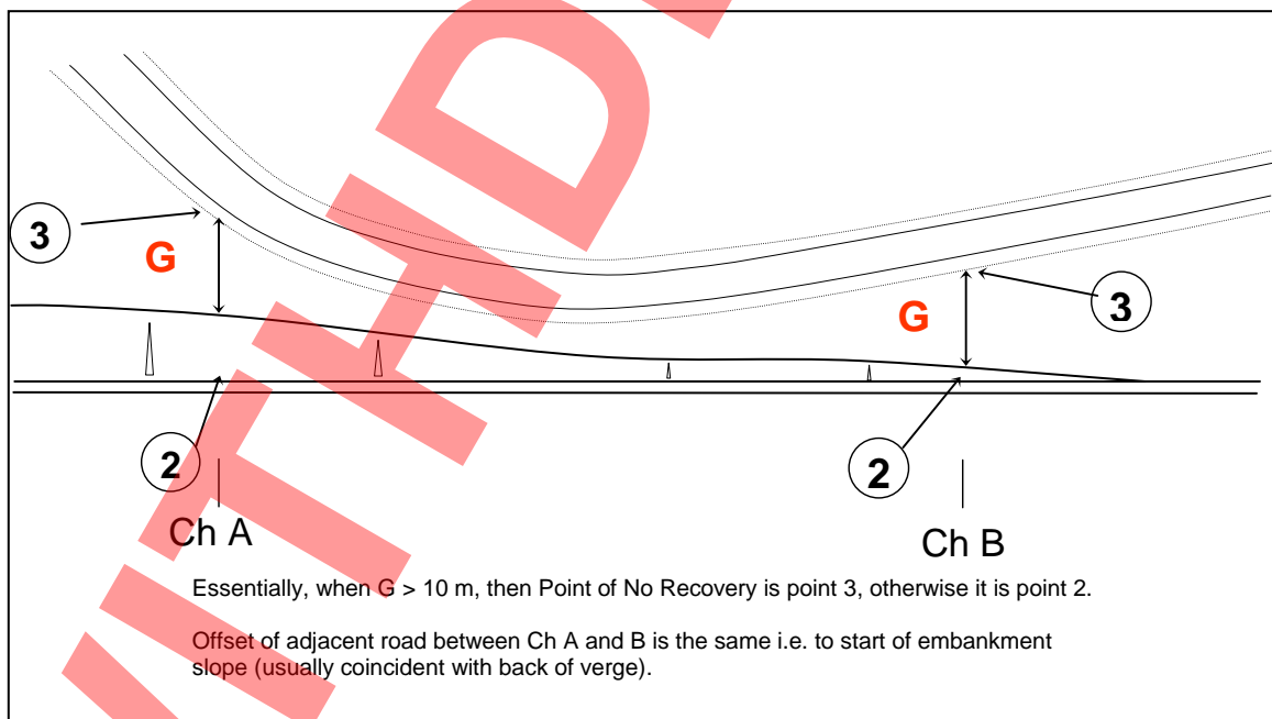
Figure 5.15 (c) Point of No Recovery for Parallel Road situation (2)
