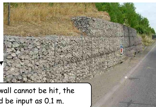
Fig 5.8-2 Gabion Wall
