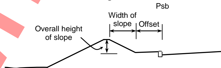
Fig 5.3.3 (b) Multiple slopes where height of false cutting is < 2.5 m
