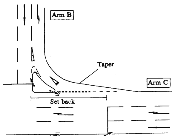
Figure 2/16: Left-Turn Slip Lane (with taper)
