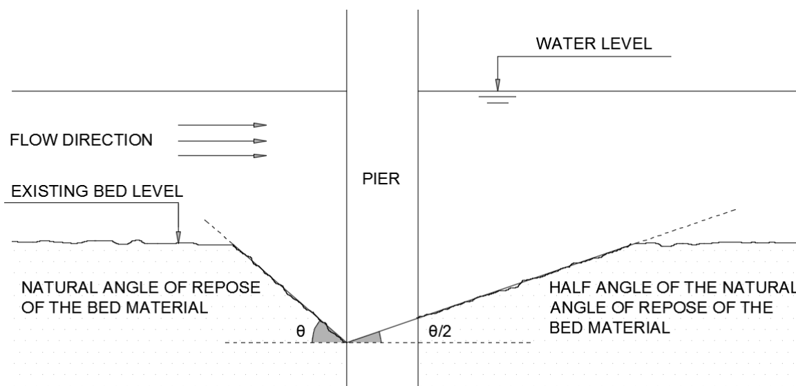
Figure 5.15.6 Typical upstream and downstream slopes of a scour hole in non-cohesive soil
