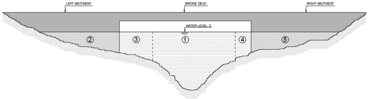
Figure B.3 Manning's application to proposed structure
